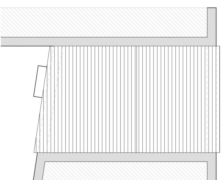
PROPOSED ROOF PLAN SCALE 1:100 @ A1
